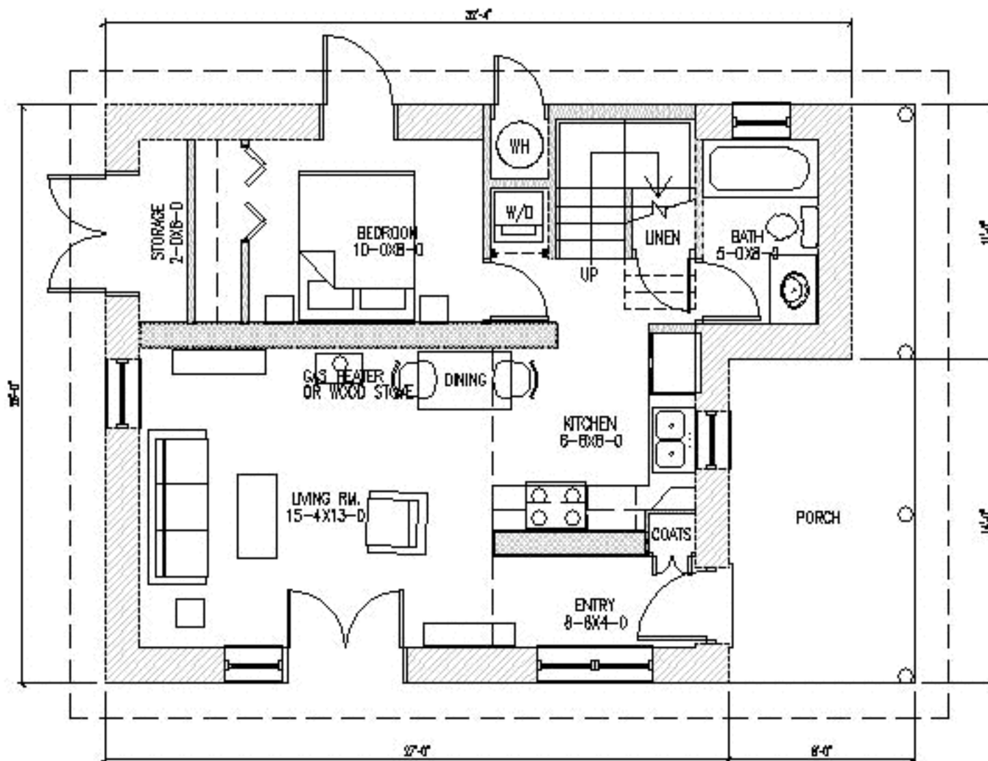
FIRST FLOOR - 734 HEATED SQ. FT. (GROSS)
